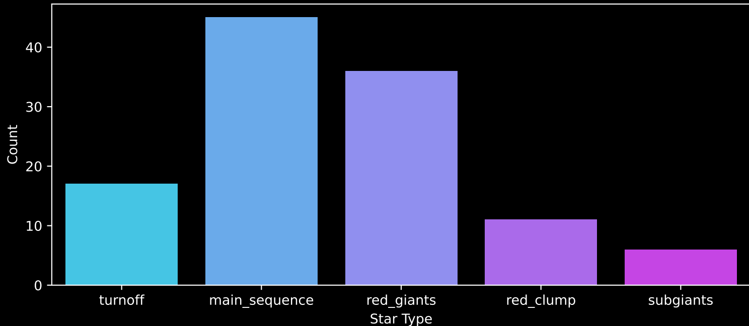
APOGEE DR17 Field: [354-03-O] Count plot of Star Type
