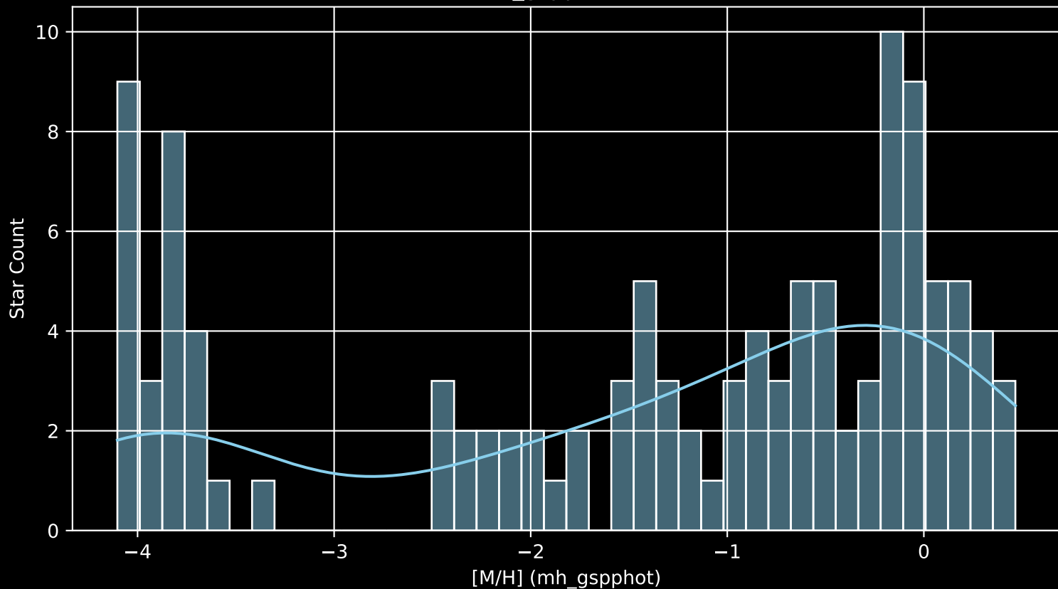
APOGEE DR17 Field: [354-03-O [M/H] (mh_gspphot) (n= 115)
