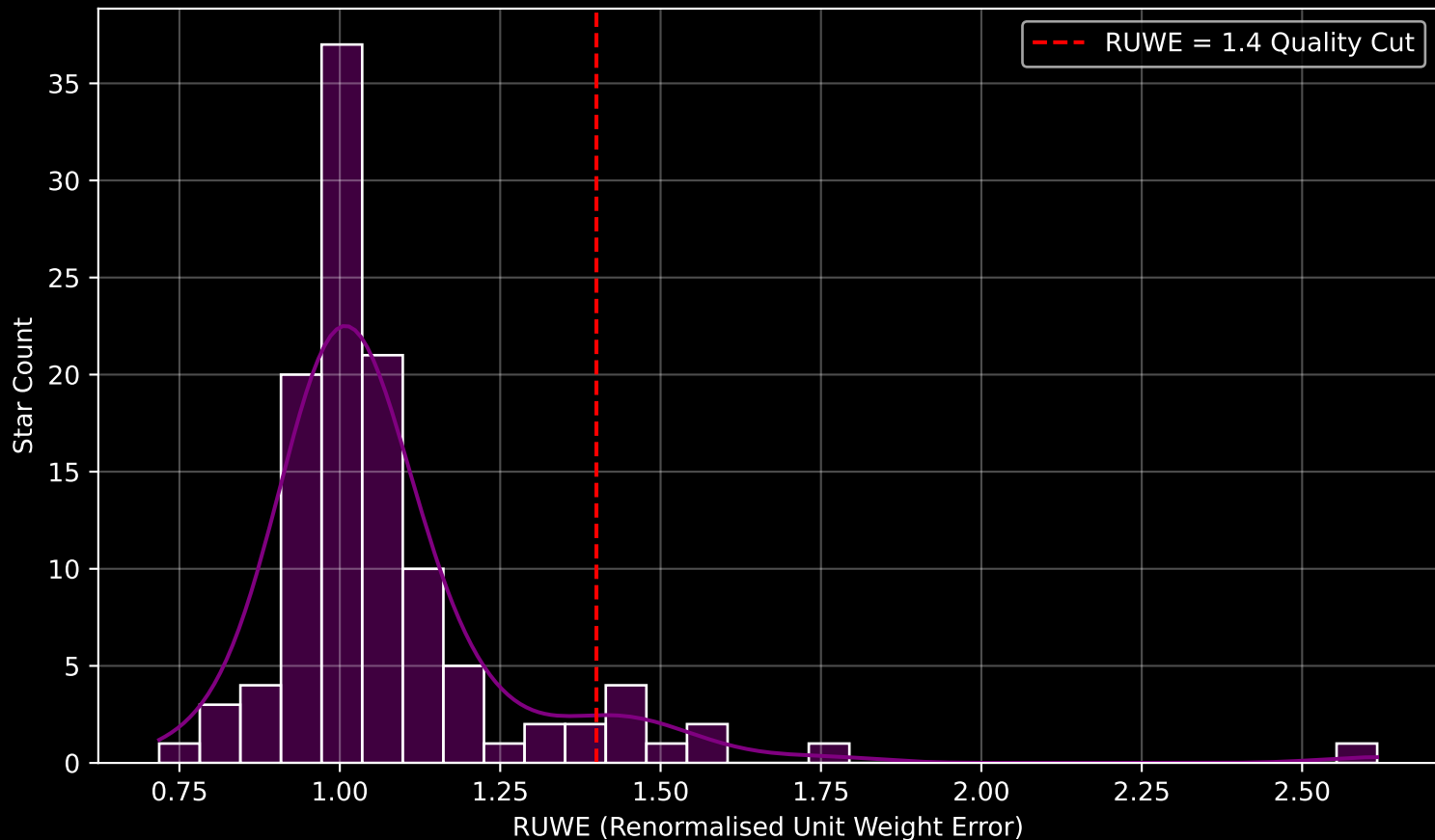
GAPOGEE DR17 Field [354-03-O] RUWE Distribution (n= 115)
