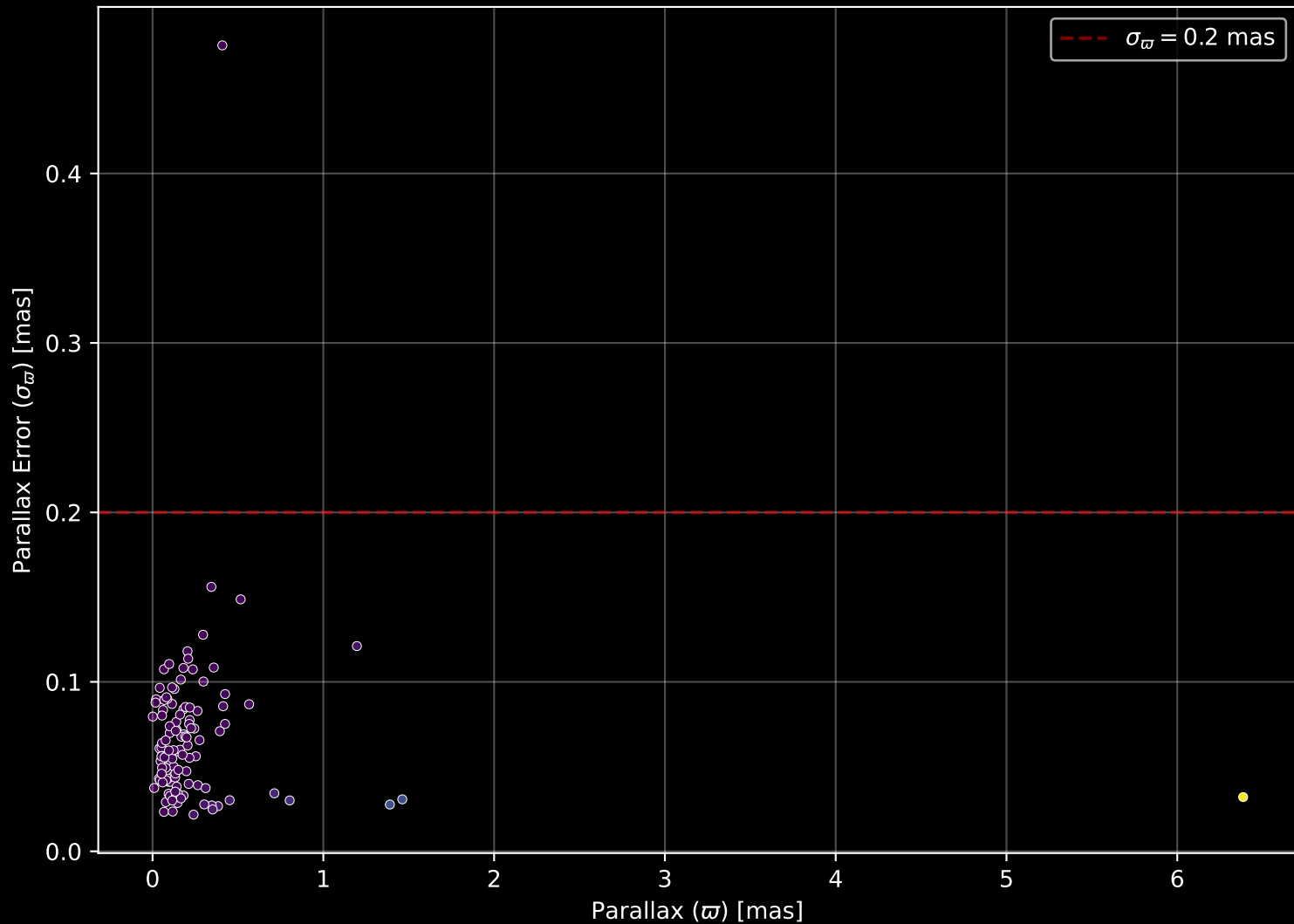
APOGEE DR17 Field: [354-03-O] Parallax Quality (n= 115)
