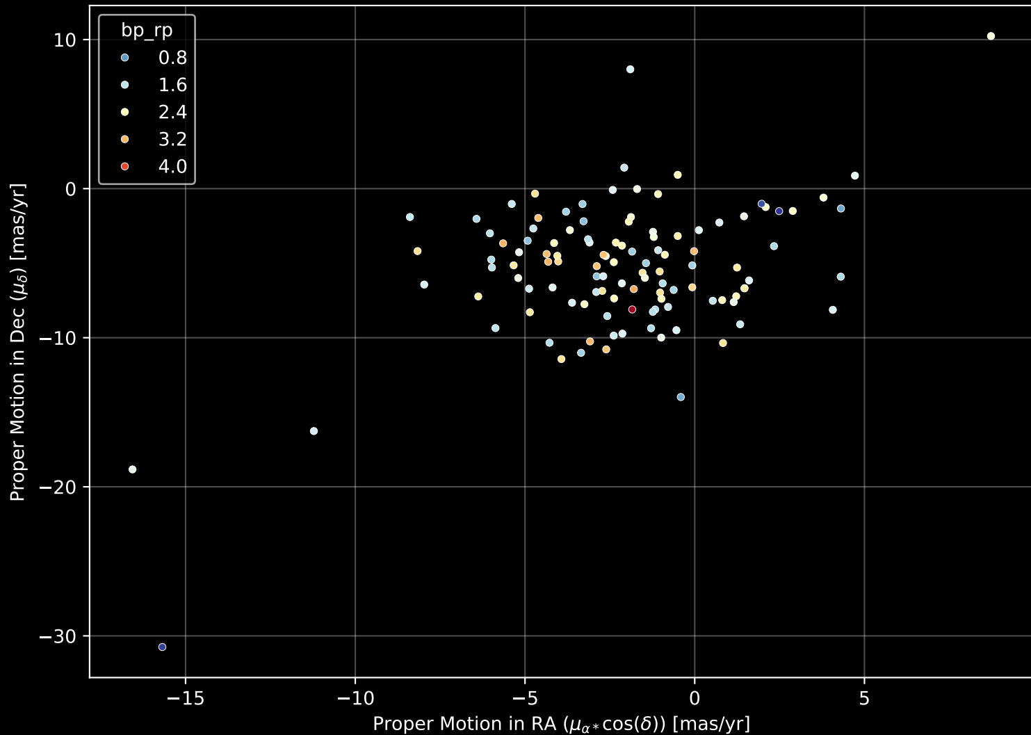
APOGEE DR17 Field: [354-03-O] Proper Motion Diagram (n= 115)
