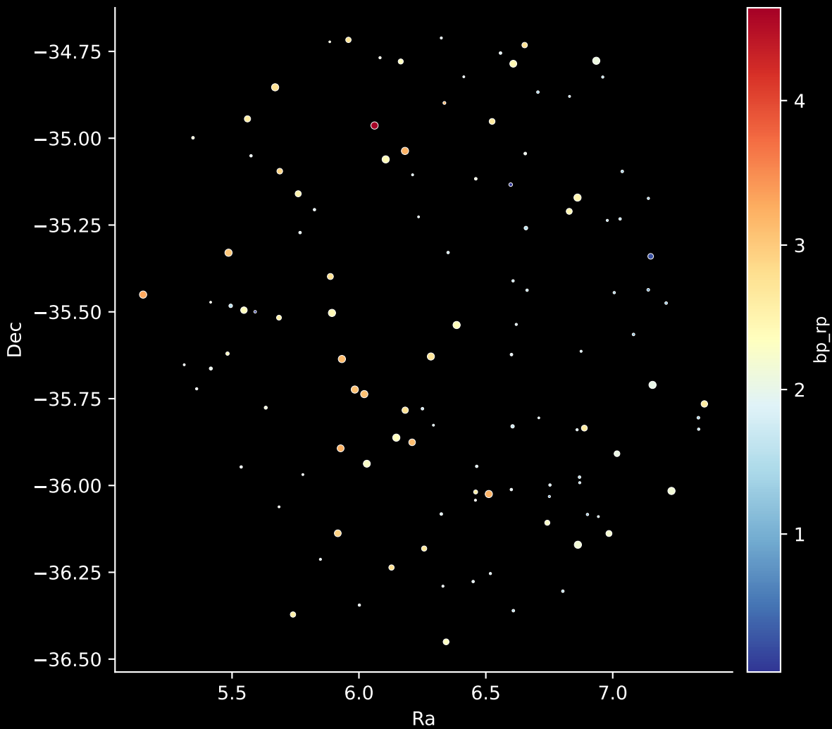
APOGEE DR17 Field: [354-03-O] Stars: 115
